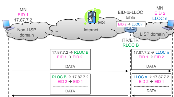
(a) Scenario 3: A MN in a non-LISP domain communicates with a MN in a LISP domain.
