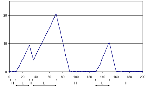
Fig. 5. A sample path of the scaled queue-length process \frac{1}{\eta} Q^\eta(t) , for \eta = 10 , in the high-low model with \lambda = 1 , a = 2 , b = \frac{1}{2}
